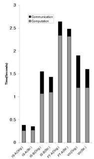
Figure 15. Application Results (8 processes, UP mode)
