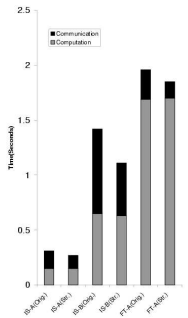
Figure 16. Application Results (16 processes, SMP mode)
