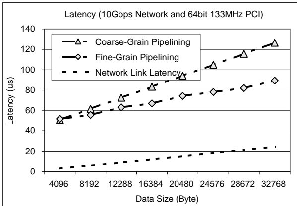
Figure 14. Latency and Bandwidth measurements on a 10Gbps network with a 64bit/133MHz I/O bus
