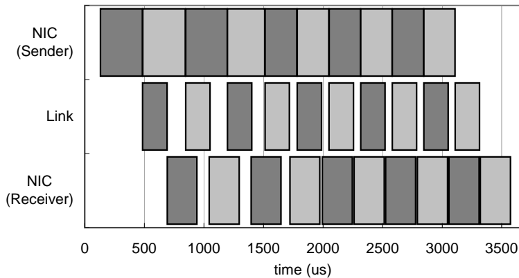
Figure 4. Time flow chart for the NIC and the link overheads for traditional UDP/IP
