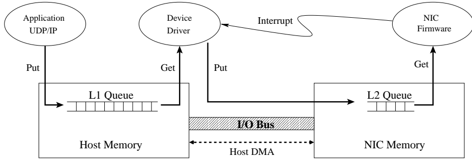
Figure 5. Two level queues to control I/O bus contention
