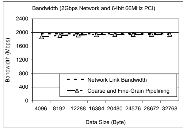
Figure 13. Latency and Bandwidth measurements on a 2Gbps network with a 64bit/66MHz I/O bus
