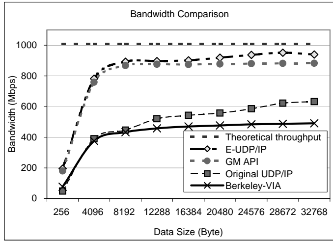
Figure 11. Bandwidth Comparison
