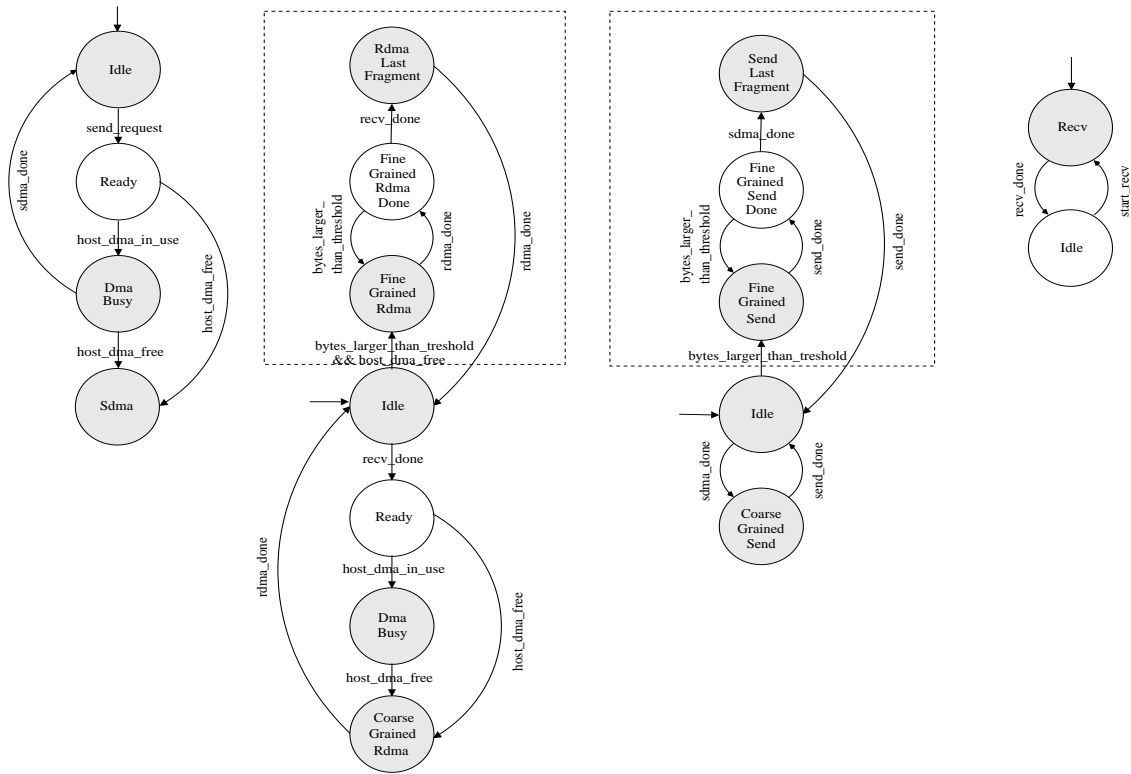
Figure 6. State Transition Model for: (a) SDMA, (b) RDMA, (c) SEND, and (d) RECV threads
