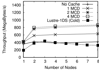
Fig. 9. Read Throughput (Varying MCDs)
