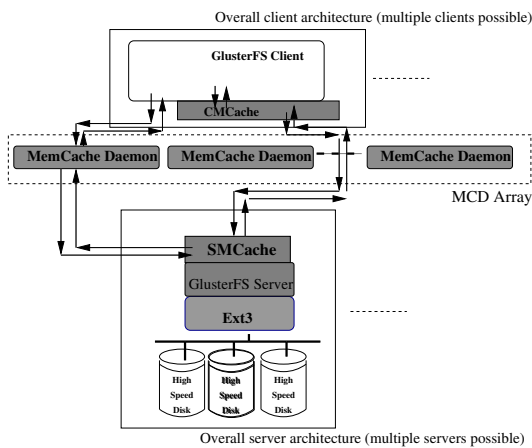
Fig. 2. Overall Architecture of the Intermediate Memory Caching (IMCa) Layer
