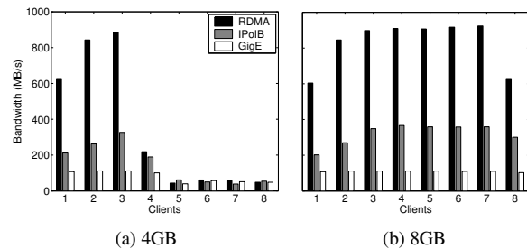
Fig. 1. Multiple clients IOzone Read Bandwidth with NFS/RDMA [9]
