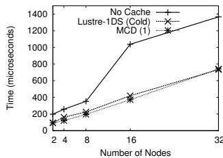
Fig. 10. Read Latency to a shared file
