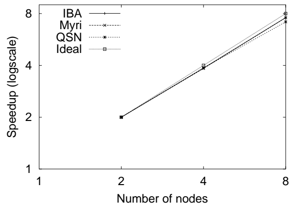
Figure 23. Speedup of Sweep3D-150
