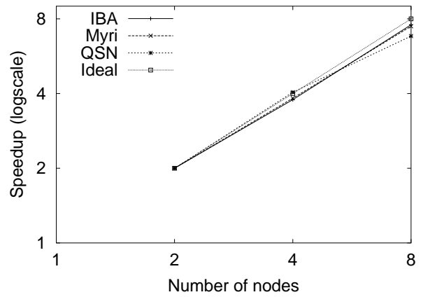
Figure 22. Speedup of Sweep3D-50
