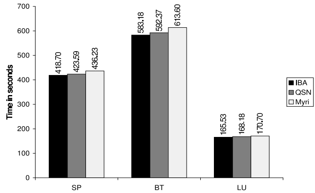
Figure 15. SP and BT on 4 Nodes and LU on 8 Nodes
