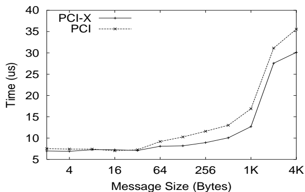
Figure 26. MPI over InfiniBand Latency (PCI vs. PCI-X)
