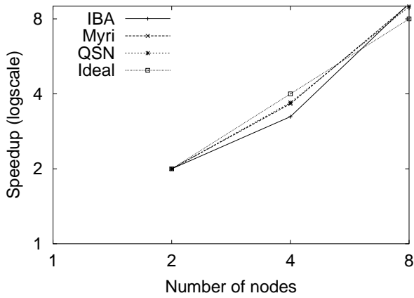
Figure 19. Speedup of CG
