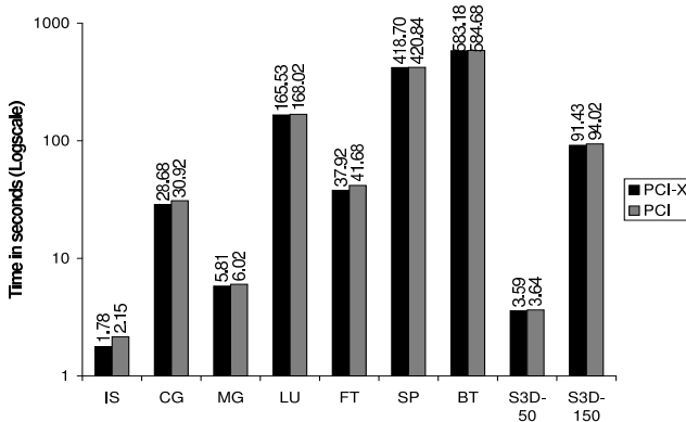
Figure 28. MPI over InfiniBand Performance (PCI vs. PCI-X)
