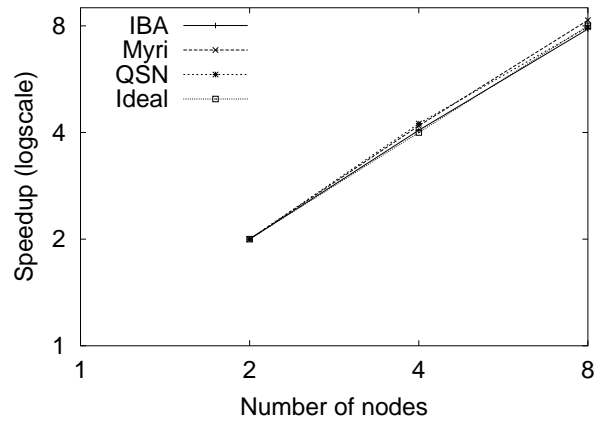
Figure 21. Speedup of LU
