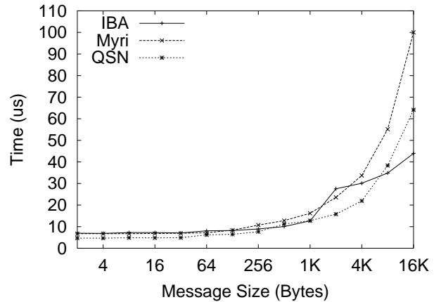
Figure 1. MPI Latency across Three Interconnects
