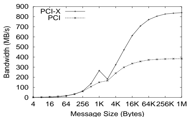
Figure 27. MPI over InfiniBand Bandwidth (PCI vs. PCI-X)
