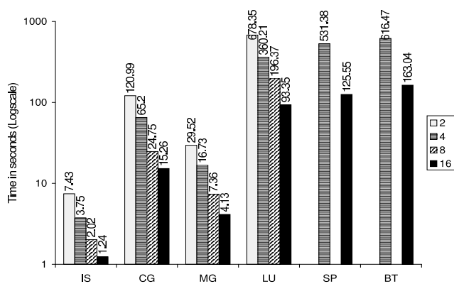
Figure 24. Scalability with System Sizes for a 16-Node System at Topspin
