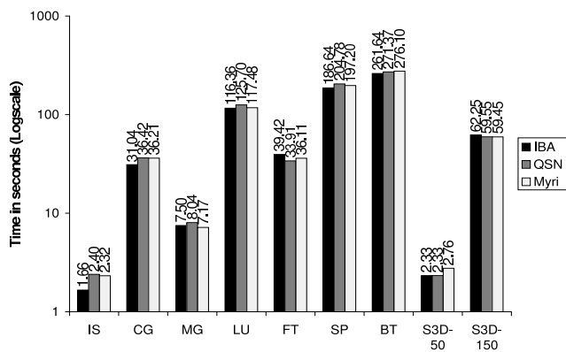
Figure 25. SMP Performance (16 Processes on 8 Nodes at OSU with block mapping)
