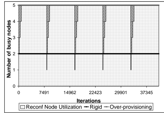
Figure 9. Node Utilization in a data-center hosting 4 web-sites with burst length (a) 512 (b) 8k
