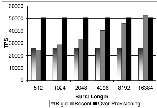
Figure 7. Impact of Burst Length (a) Number of co-hosted web-sites = 3 (b) Number of co-hosted web-sites = 4
