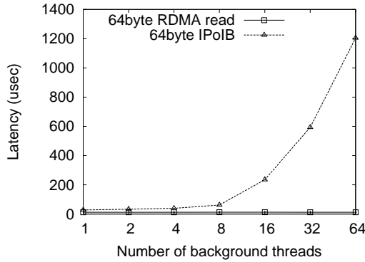
Figure 6. Performance of IPoIB and RDMA Read with background threads: (a) Latency and (b) Bandwidth
