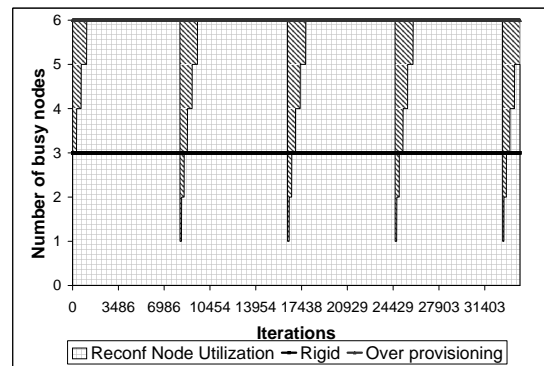
Figure 8. Node Utilization in a data-center hosting 3 web-sites with burst length (a) 512 (b) 8k
