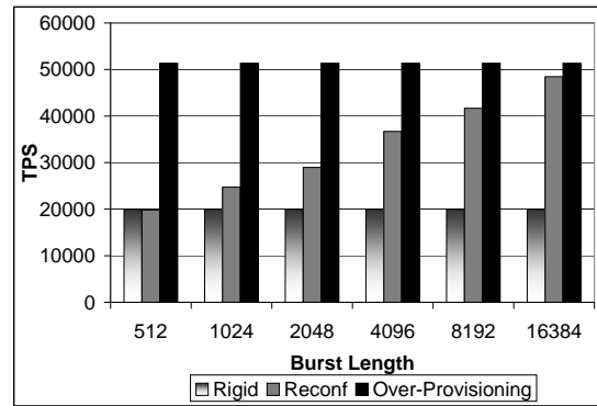
Figure 7. Impact of Burst Length (a) Number of co-hosted web-sites = 3 (b) Number of co-hosted web-sites = 4
